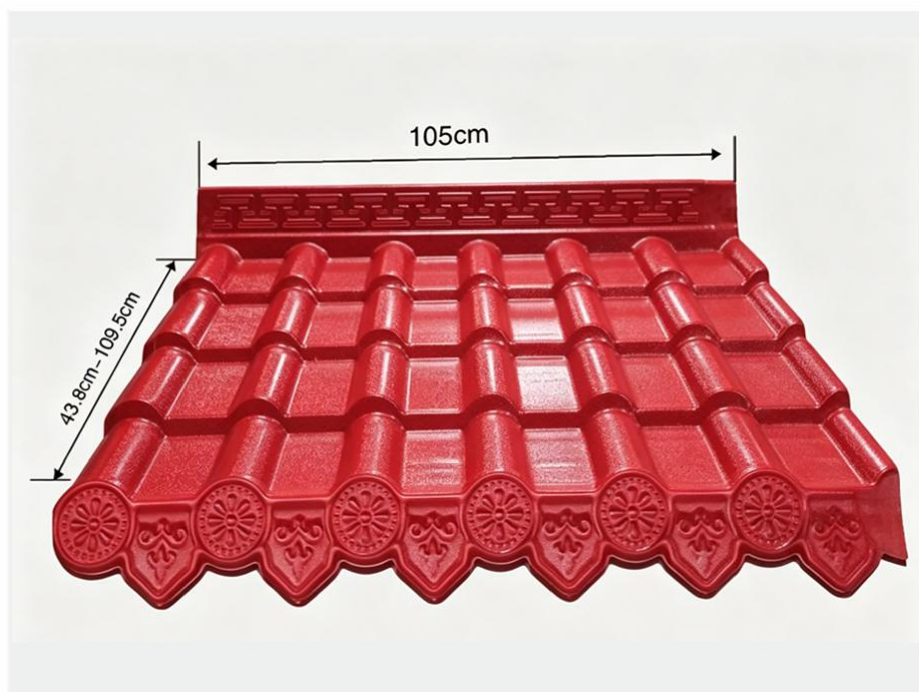
Specifications of Integrated Resin Tile
